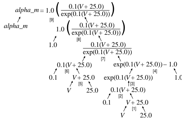
FIGURE 23: The tree form of Equation (45), in which each non-leaf node is obtained by the application of a single operator to its children. Each operator is represented by a number in square brackets. The effect of each operator is discussed in the text.
